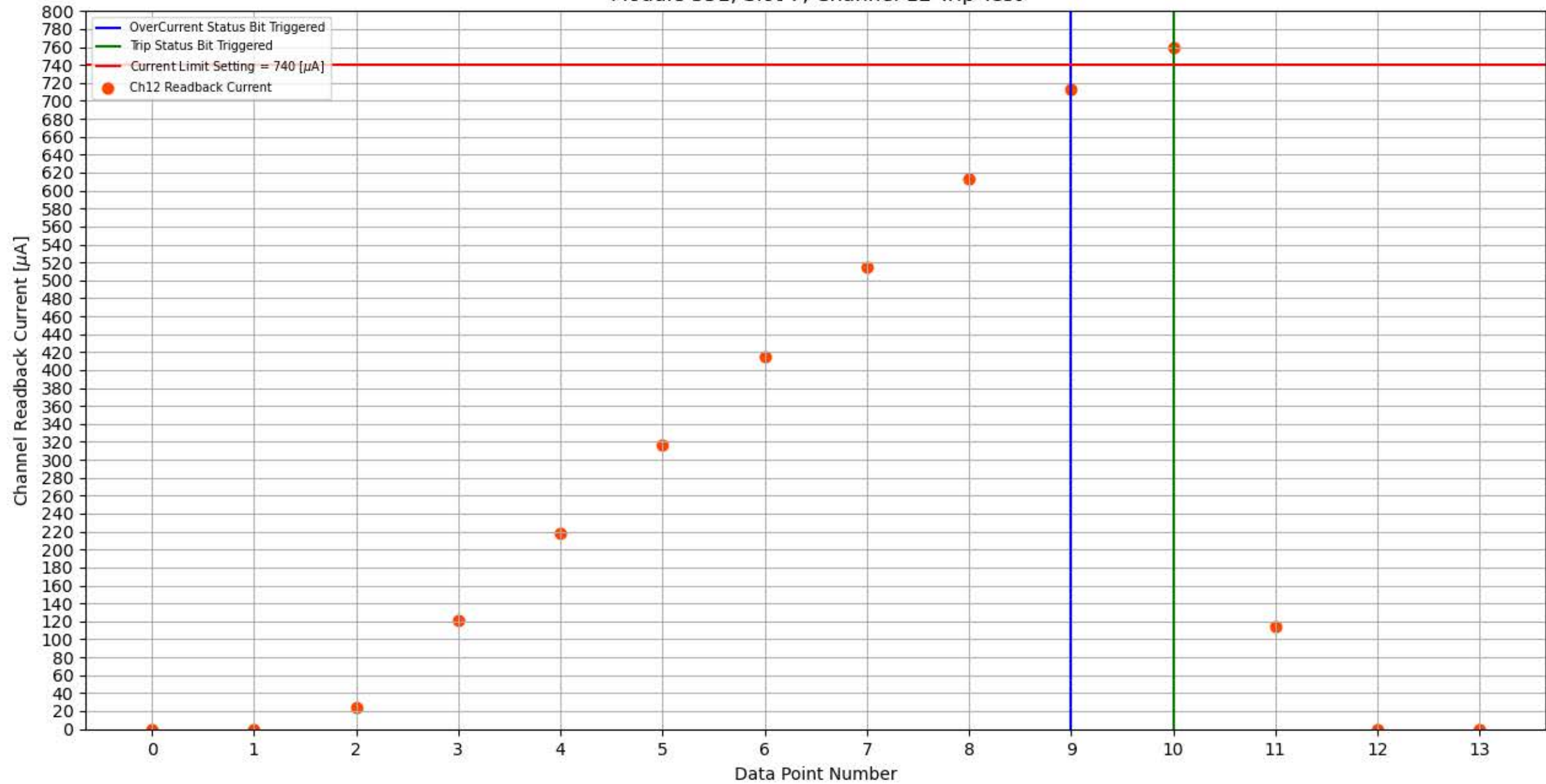
Module 351, Slot 7, Channel 12 Trip Test
