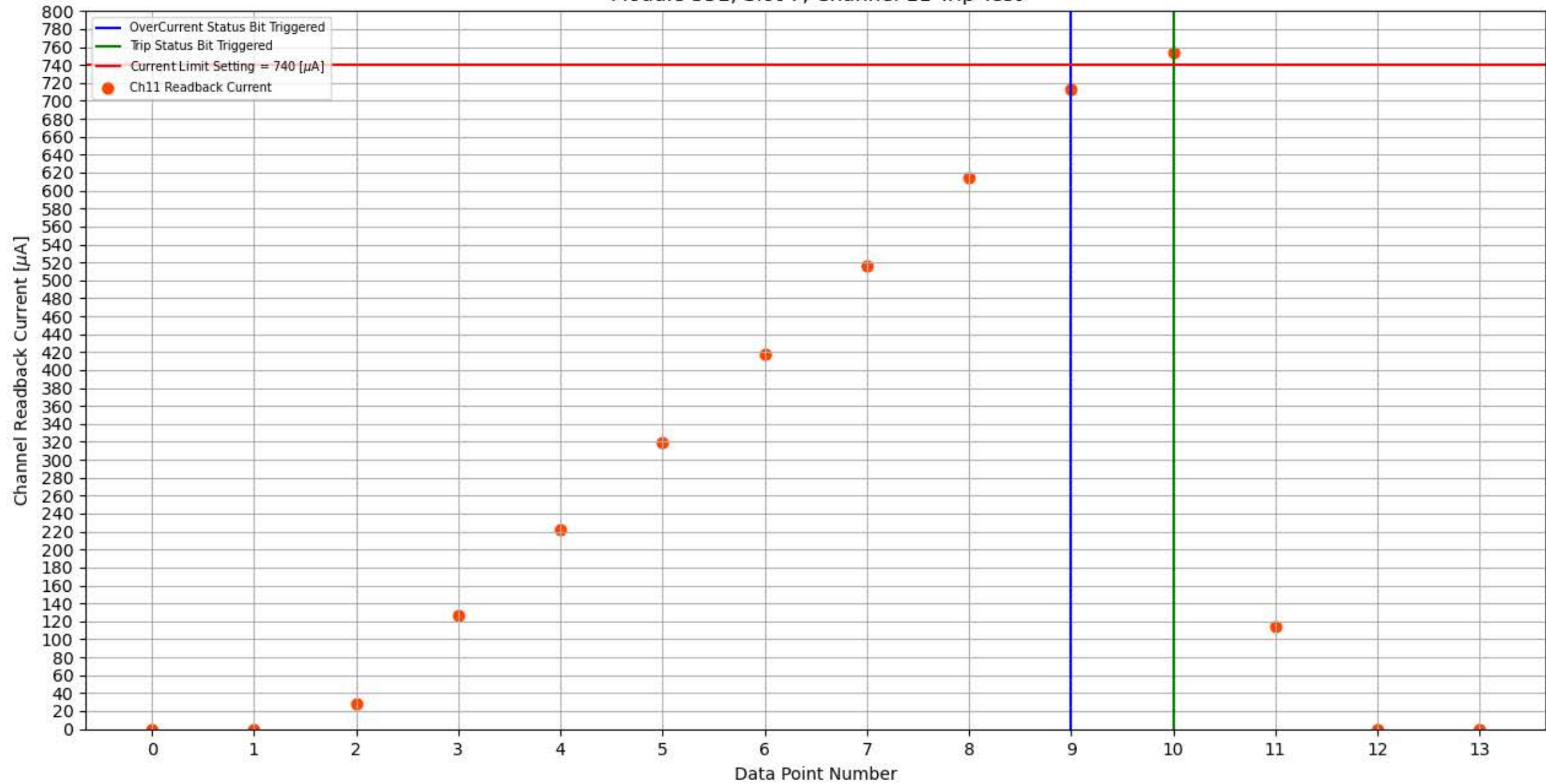
Module 351, Slot 7, Channel 11 Trip Test
