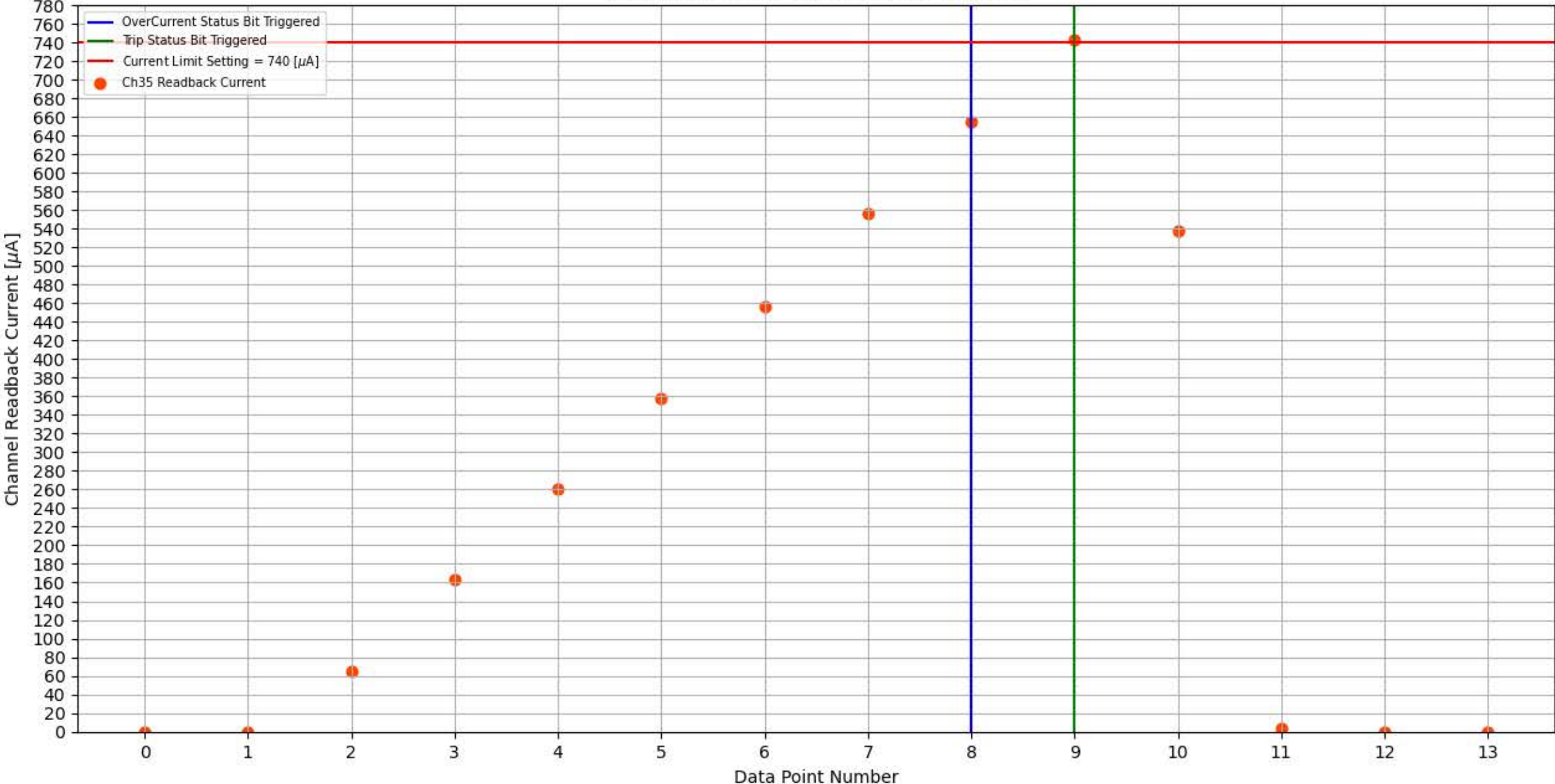
Module 351, Slot 7, Channel 35 Trip Test
