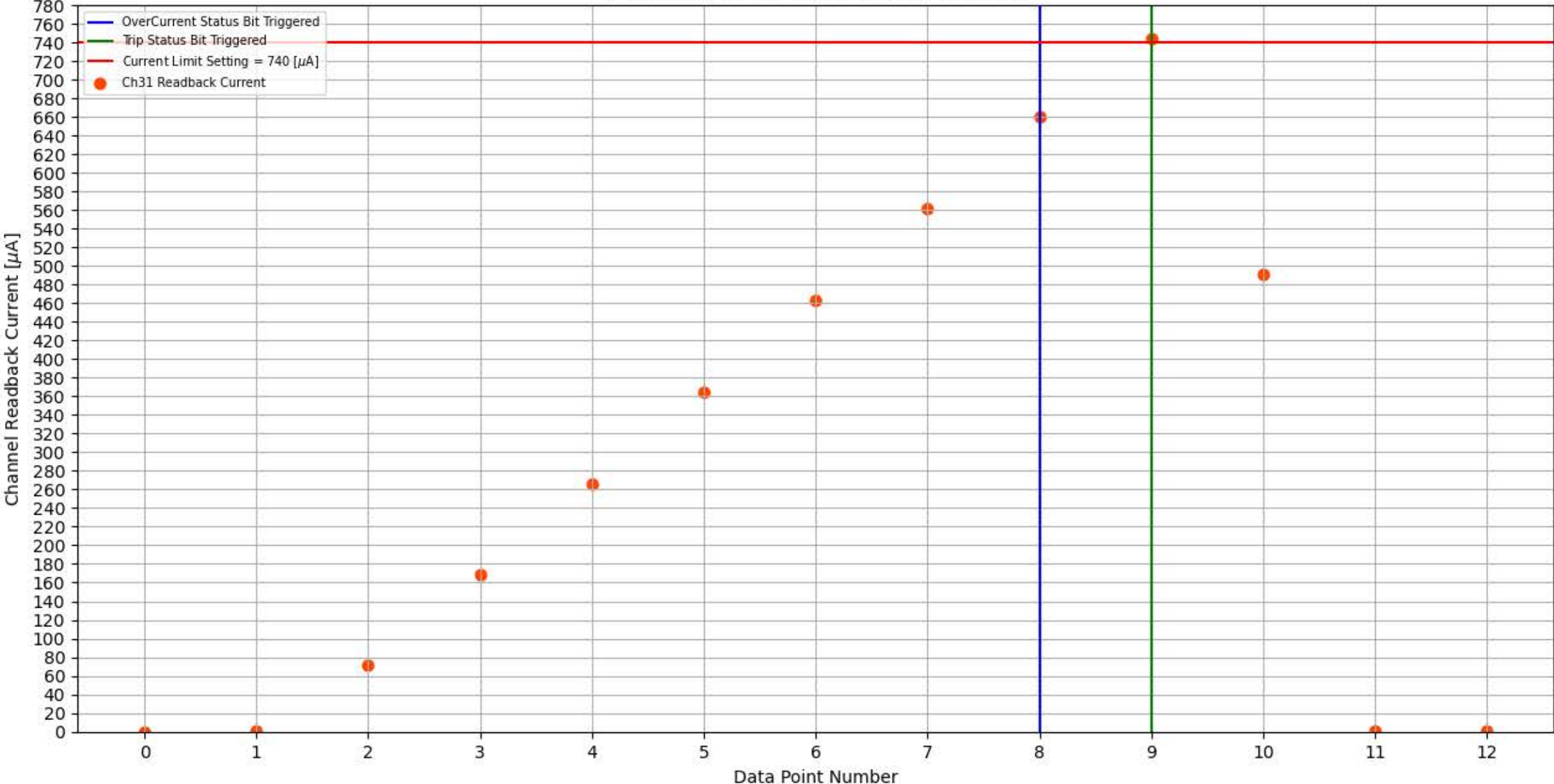
Module 351, Slot 7, Channel 31 Trip Test
