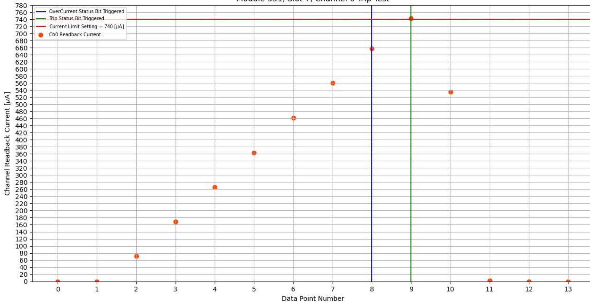
Module 351, Slot 7, Channel 0 Trip Test
